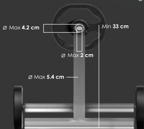
T-shaped cover reel frames Required dimensions
